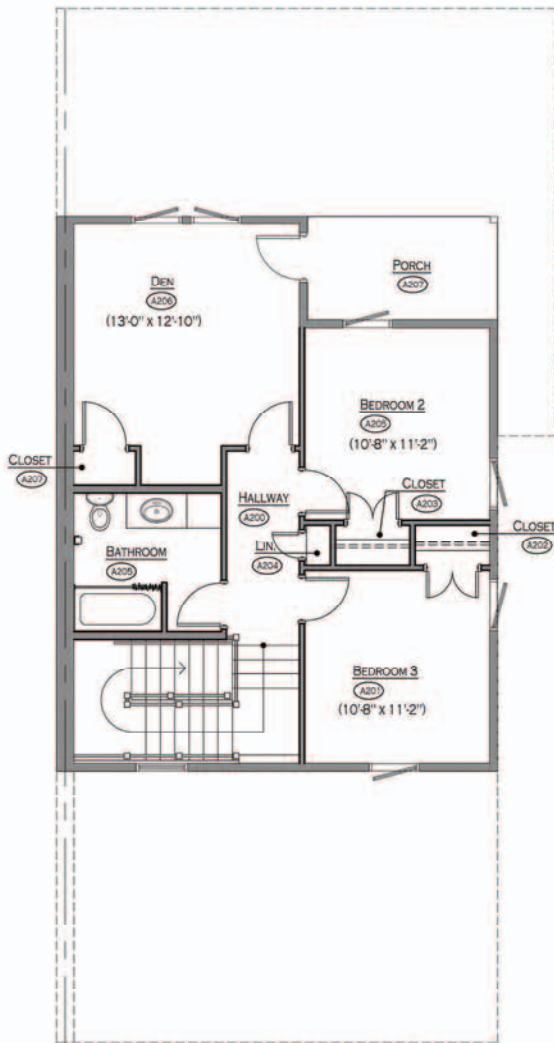
2 SECOND FLOOR PLAN A-200 1/4"=1'-0"
