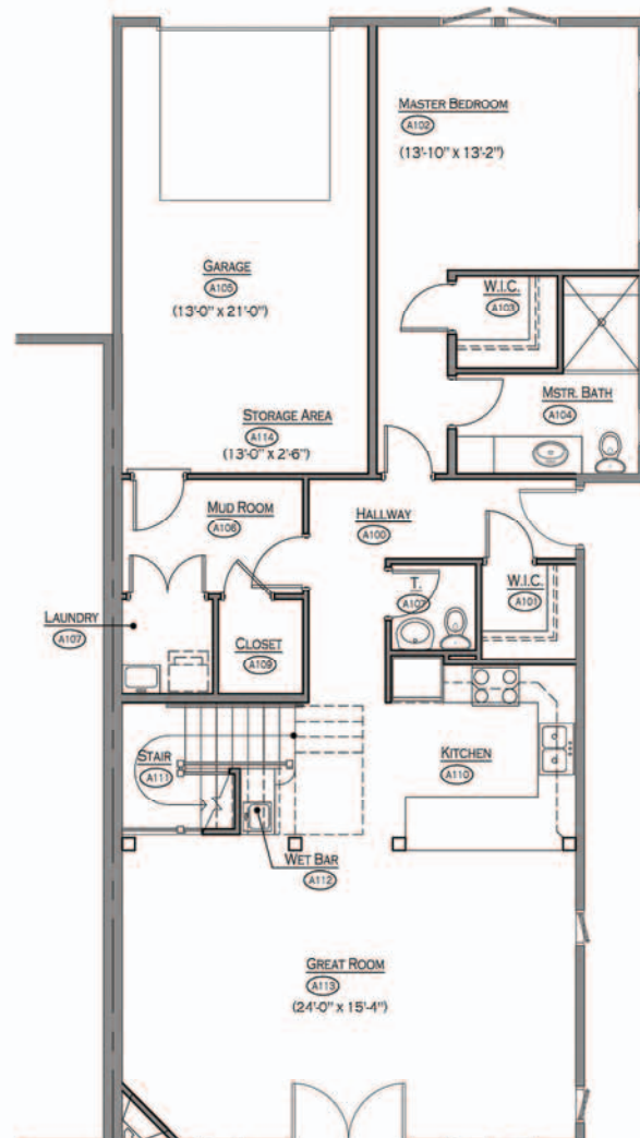
1 FIRST FLOOR PLAN A-200 1/4"=1'-0"
